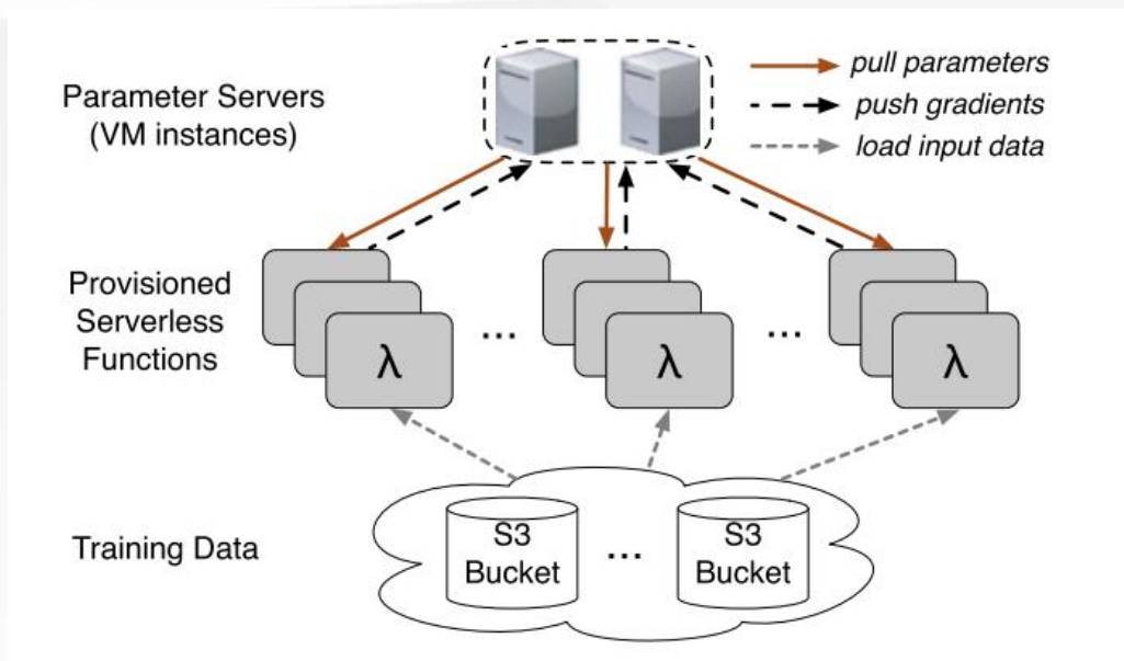
Serverless model training
