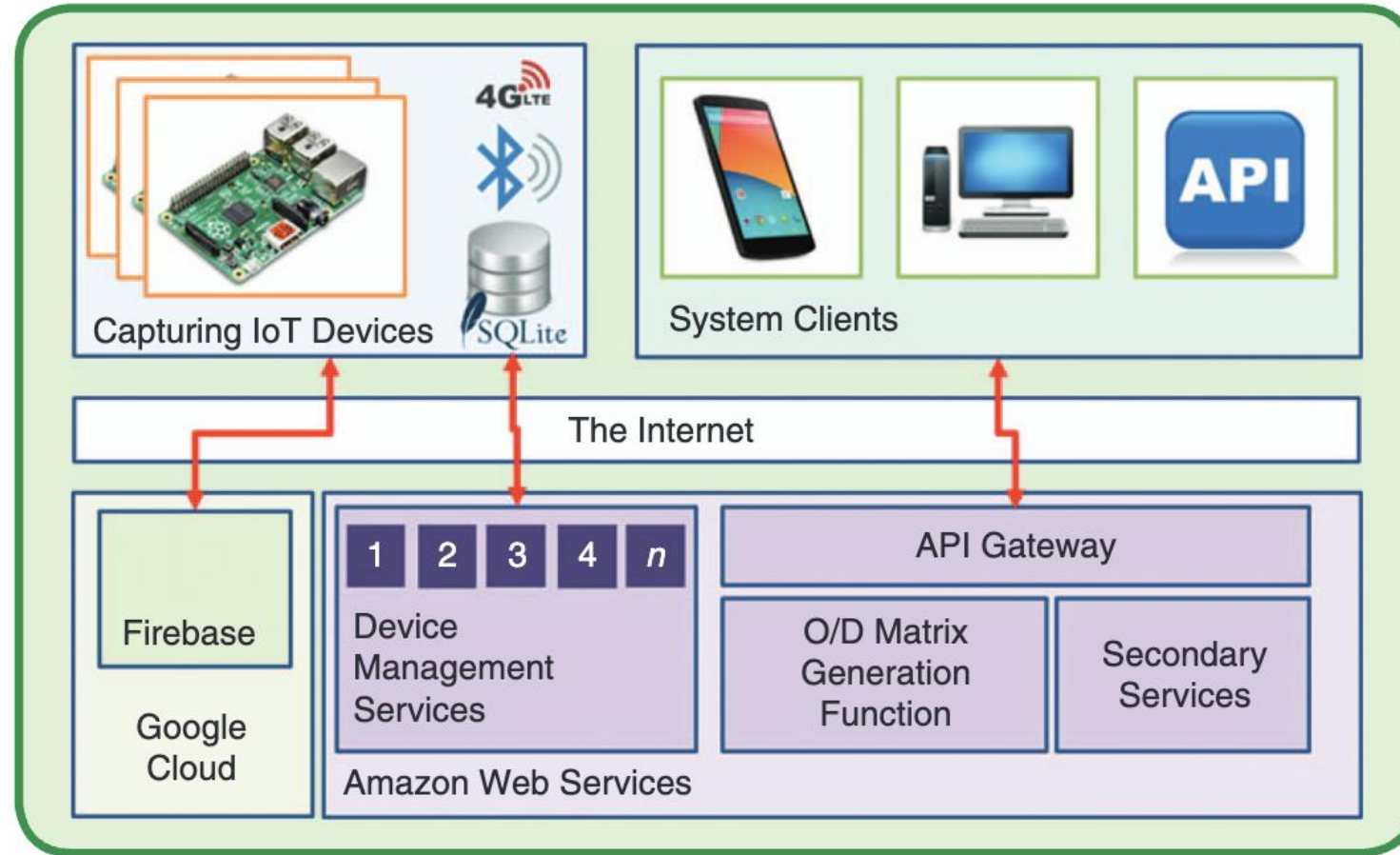
Serverless based IoT architecture
