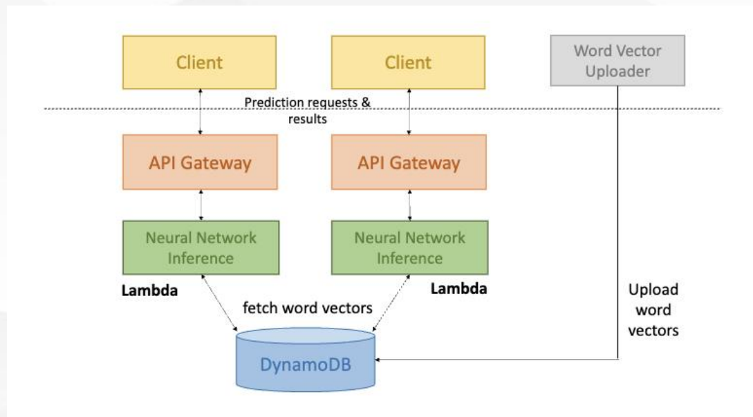
Serverless model inference
