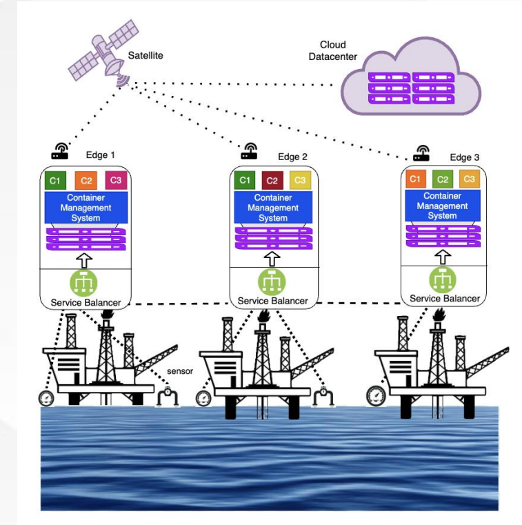
An oil and gas field management system
